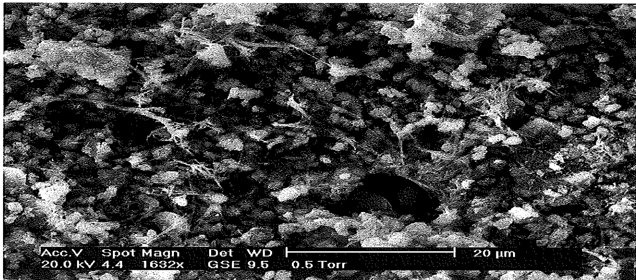
Plate 2: Hydraulic lime mortar NHL2 (Environmental Scanning Electron Microscope) [vi]
