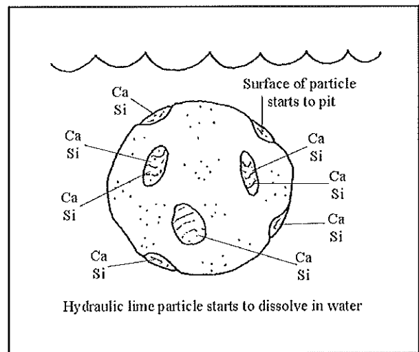
Figure 4: Stage 2 of hydration process – Hydraulic lime particle starts to dissolve (Forster)
